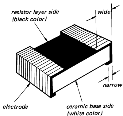
Resistor
