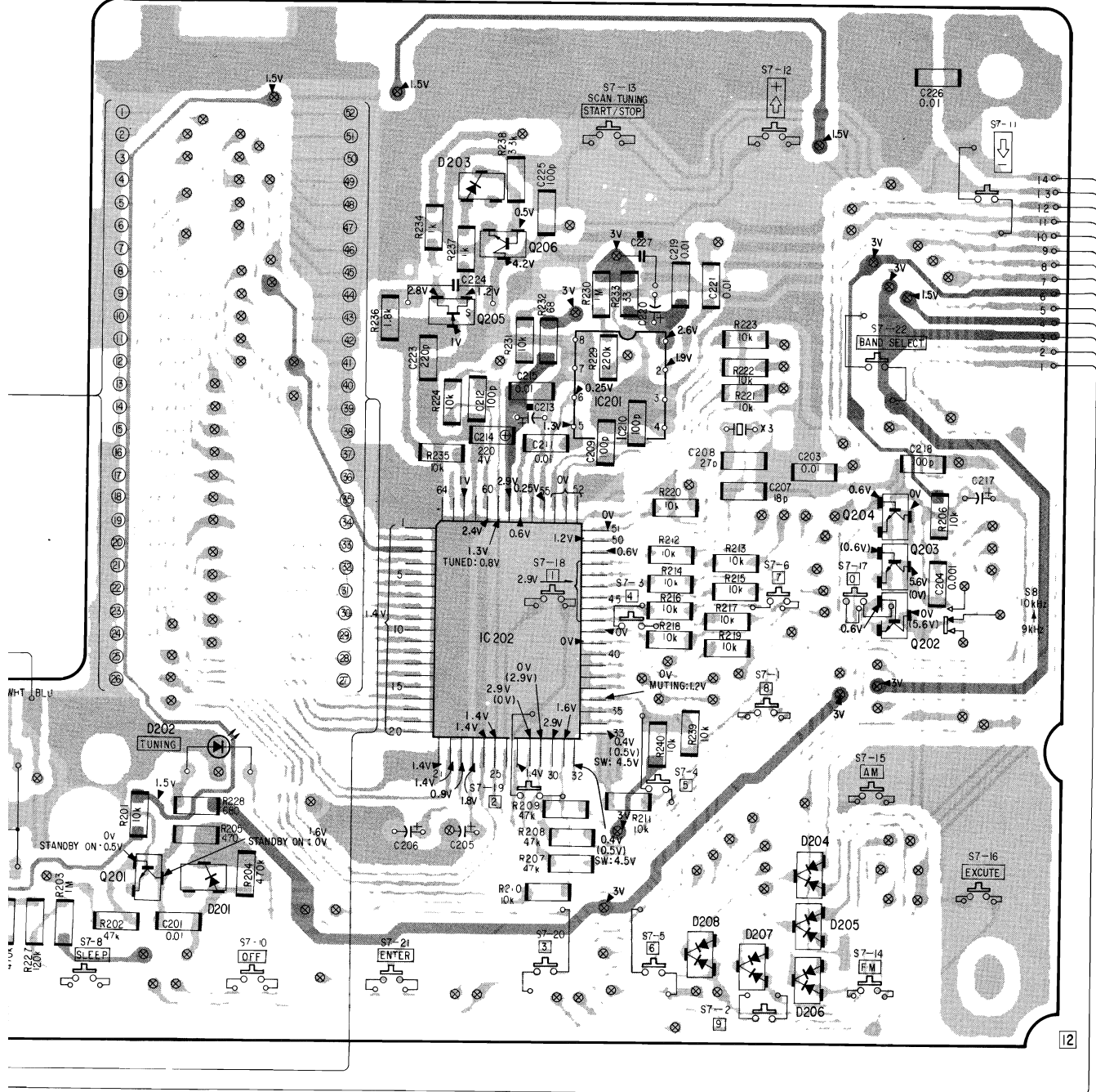
[SWITCH BOARD]
