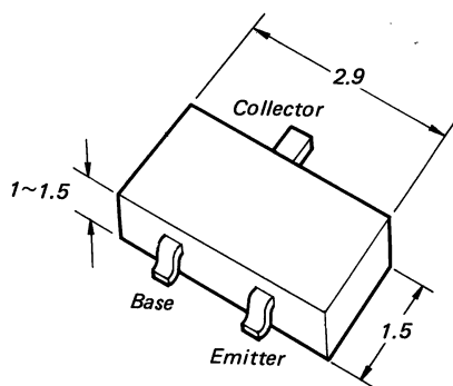
Transistor
